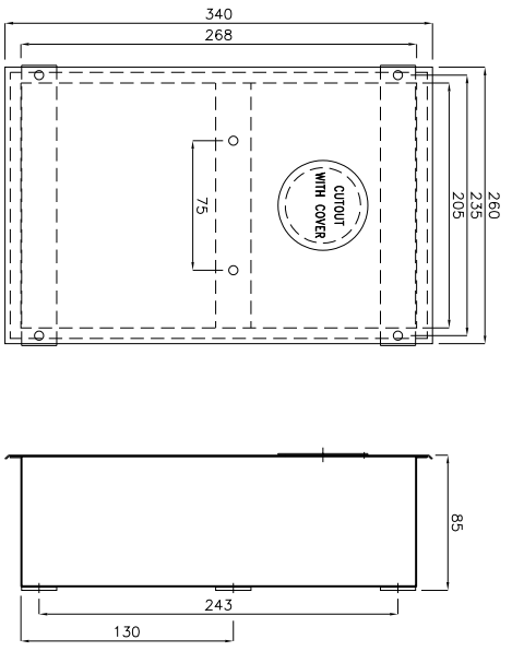
SS COVER WITH M.S. BOX CUTOUT SIZE IN WALL : (W) 380 x (H) 180 x (d)85mm
